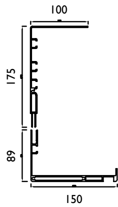
TRAVE
